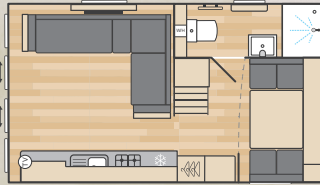
S-POD 6 - day 21' x 12' - 6 berth
